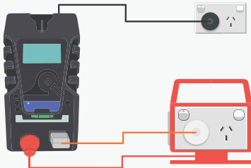
Testing Portable RCDs with physical switches
